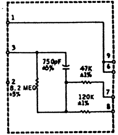
7.5CCIR/15CCIR REPRODUCE EQUALIZER Q2-96113-02
