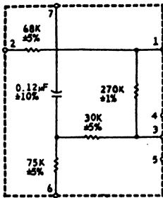
7.5 NAB/15 NAB RECORD EQUALIZER Q2-96121
