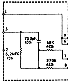
3.75(200µSEC.) 7.5NAB REPRODUCE EQUALIZER Q2-96114-02
