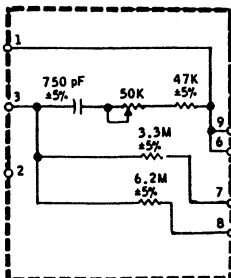
7.5 NAB/15NAB REPRODUCE EQUALIZER 96111-03
