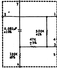
3.75-7.5 NAB RECORD EQUALIZER A-96120
