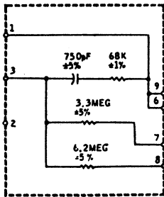
7.5NAB/15NAB REPRODUCE EQUALIZER Q2-96111-02
