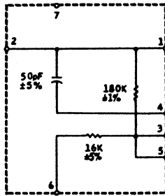
7.5 CCIR/15 CCIR RECORD EQUALIZER Q2-96123
