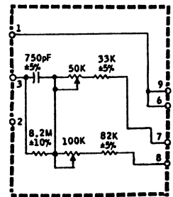
7.5 CCIR/15CCIR REPRODUCE EQUALIZER 96113-03
