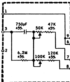
3.75 (120µSEC.) 7.5 NAB REPRODUCE EQUALIZER 96110-03
