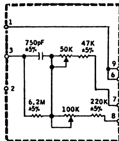
3.75 (200µSEC.) 7.5 NAB REPRODUCE EQUALIZER 96114-03
