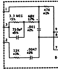
7.5NAB/15AME REPRODUCE EQUALIZER Q2-96112-02
