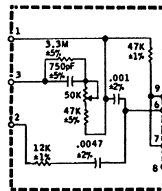
7.5 NAB/15 AME REPRODUCE EQUALIZER 96112-03
